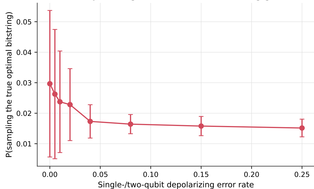
E15: QAOA( p=1 ) degradation under increasing gate noise
