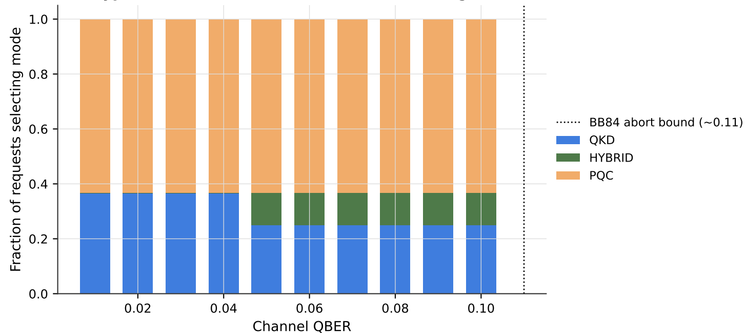
Crypto-mode selection shift under increasing QBER
