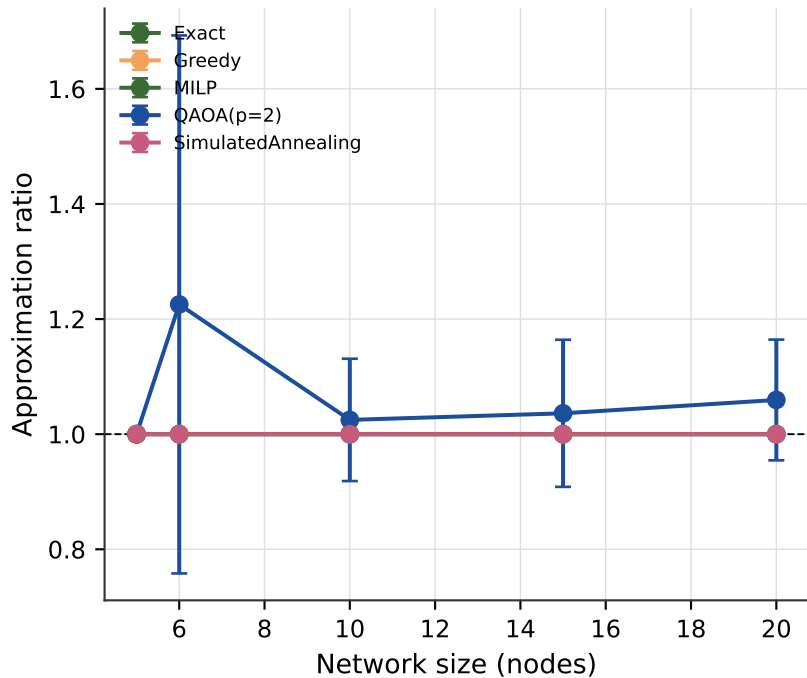
(a) Solution quality vs. network size
