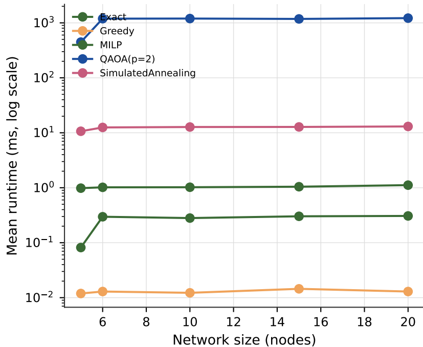
(b) Runtime scaling vs. network size
