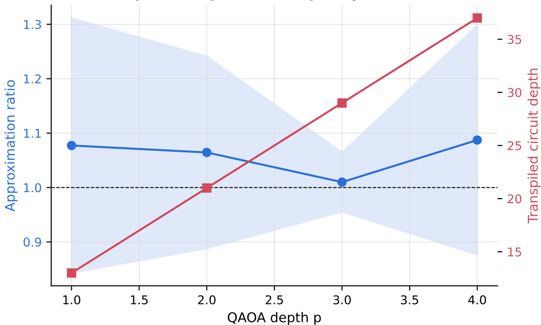
QAOA depth sweep: solution quality vs. circuit cost
