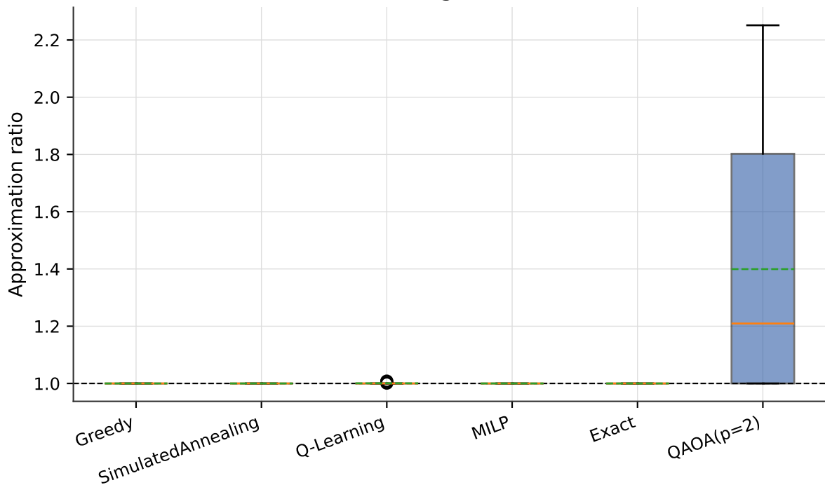
QAOA vs. RL (Q-learning) vs. classical baselines
