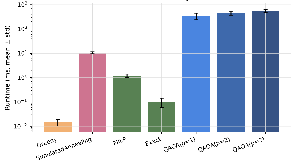
Solver runtime comparison
