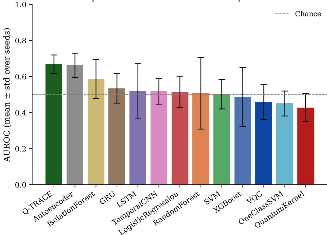
Zero-Day Detection AUROC Across Independent Seeds
