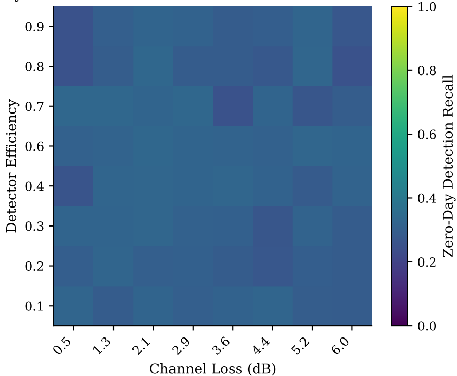
Zero-Day Detection Recall vs. Channel Loss and Detector Efficiency
