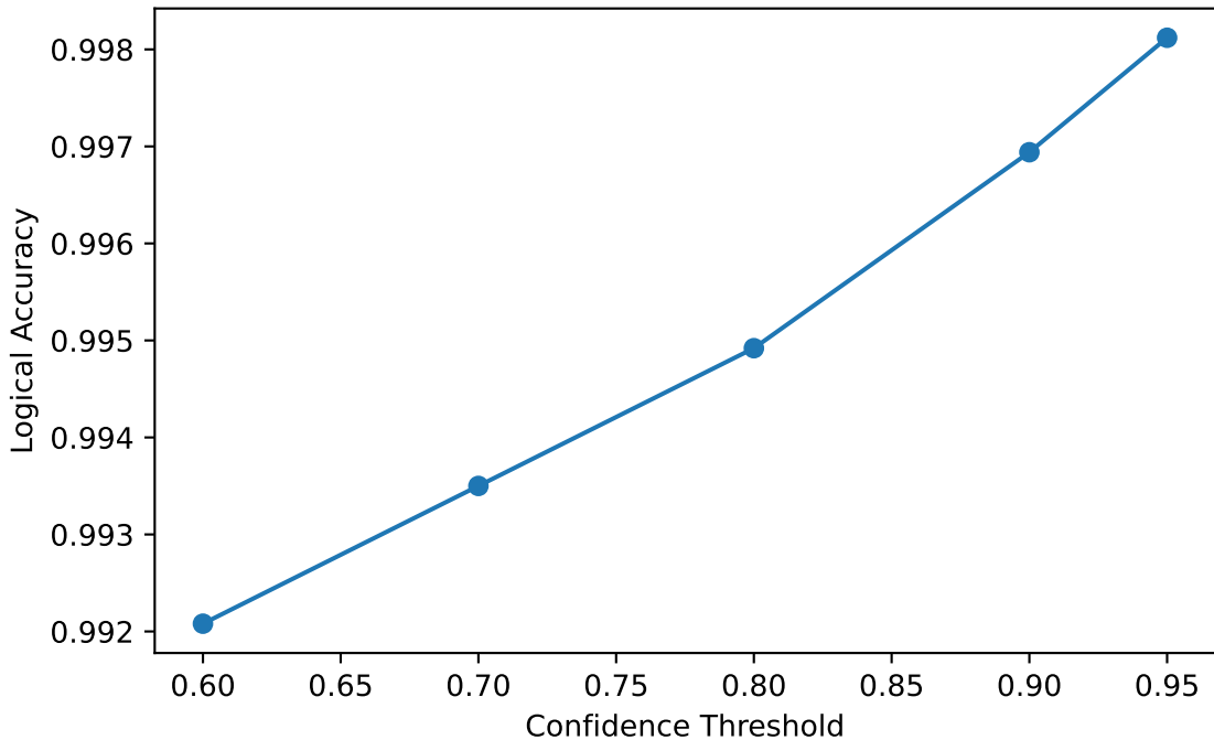
Adaptive Neural/PyMatching Routing
