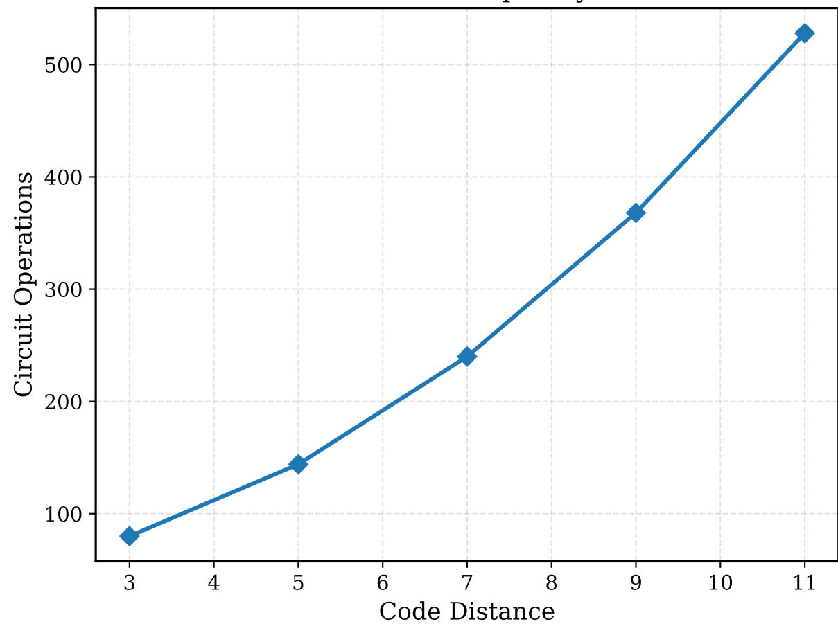
Circuit Complexity
