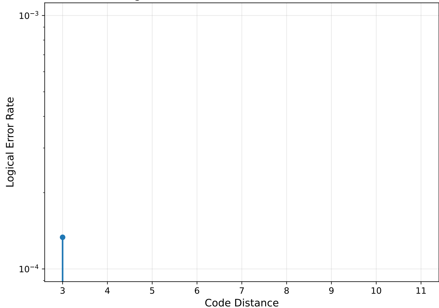
Logical Error vs Distance (Noise=0.0001)
