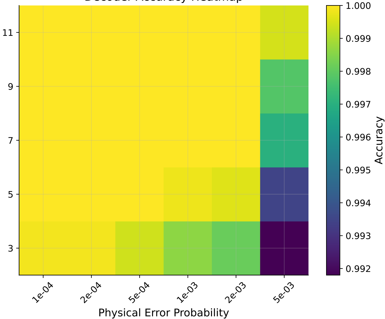
Decoder Accuracy Heatmap
