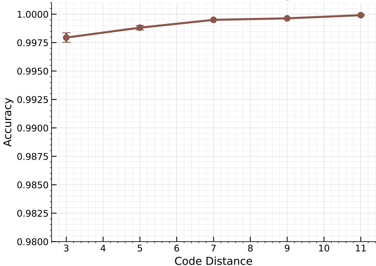
Baseline Decoder Accuracy
