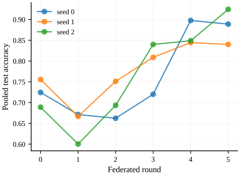
QFL (FedAvg) training convergence
