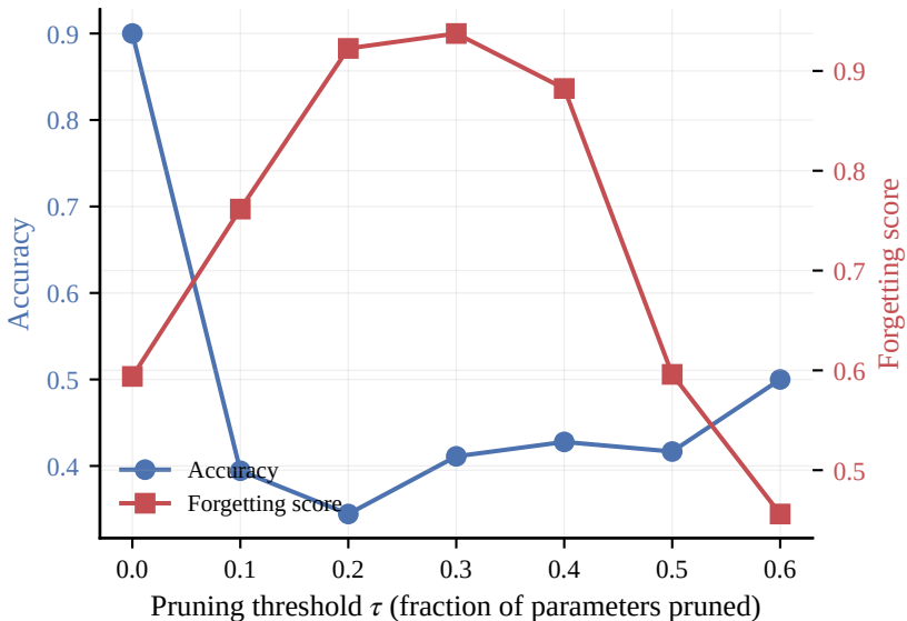
Hyperparameter sensitivity: pruning threshold \tau (QFL-EWP)
