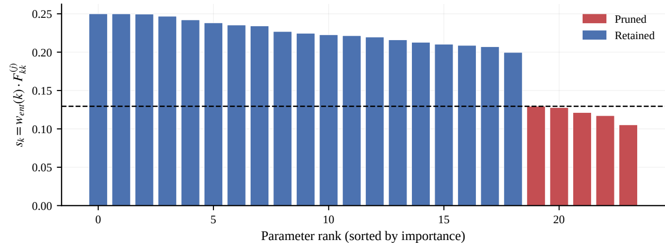
Parameter importance ranking (EWP pruning scores)
