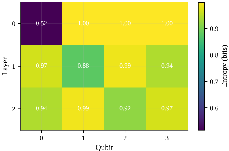
Per-gate entanglement weight w_{ent}(k) (single-qubit von Neumann entropy)
