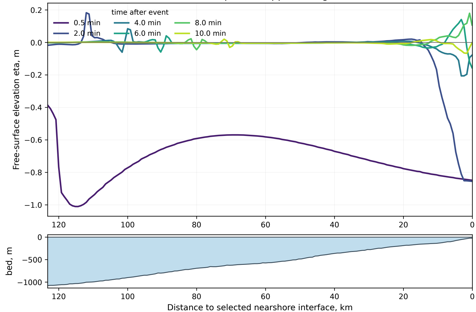
R10 h400 wave profiles approaching Kamaishi
