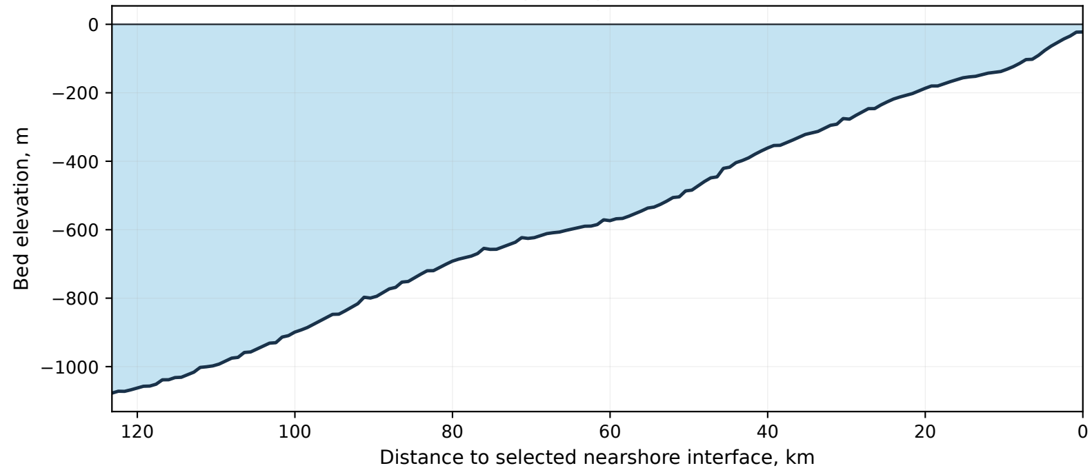
Longitudinal bathymetry sampled from the R10 h400 mesh
