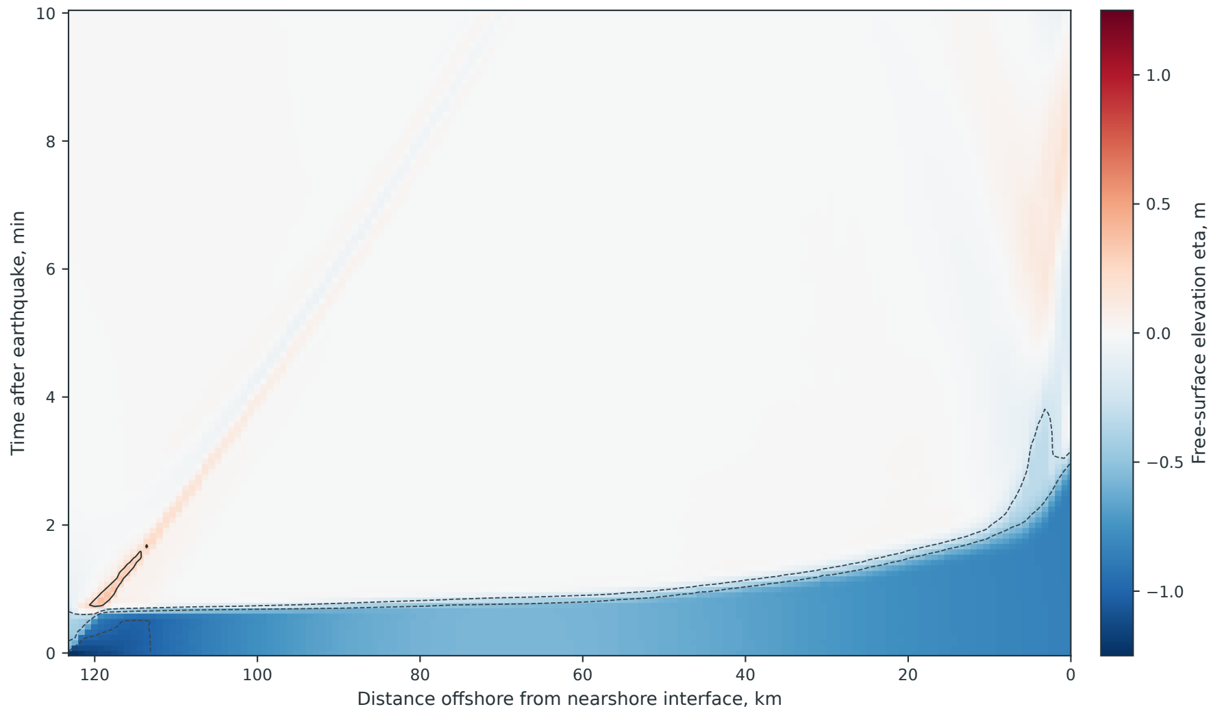
Simulated free-surface evolution toward Kamaishi
