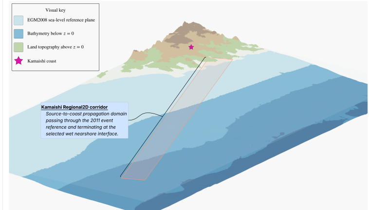
B. Oblique Kamaishi corridor bathymetry/topography. ETOPO 2022, EGM2008, QGIS/GDAL, Blender 5.2 Eevee; 4× vertical exaggeration.
