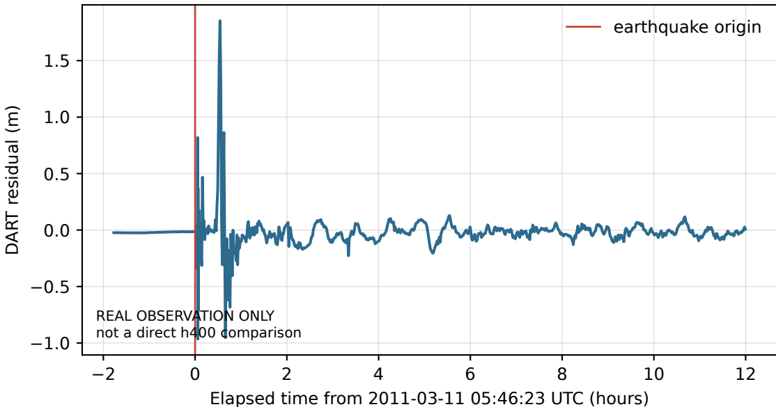
NOAA/NCEI DART 21418 observed residual waveform
