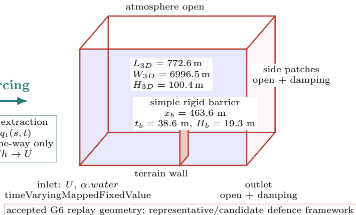
(b) Local3D computational domain
