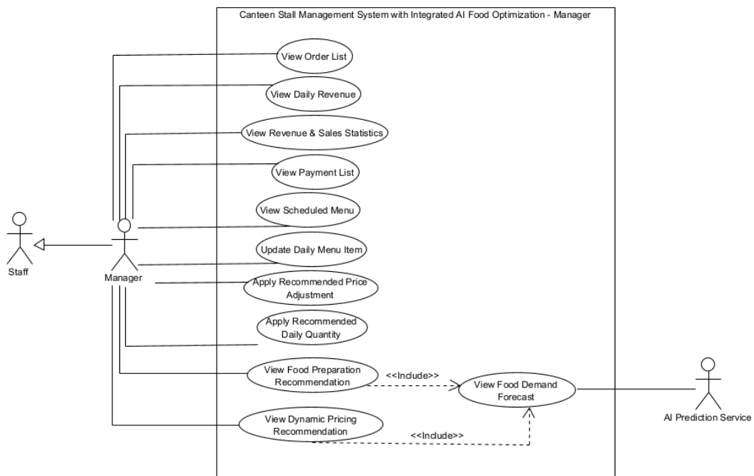
Figure 3. Use Case Diagram for Manager
