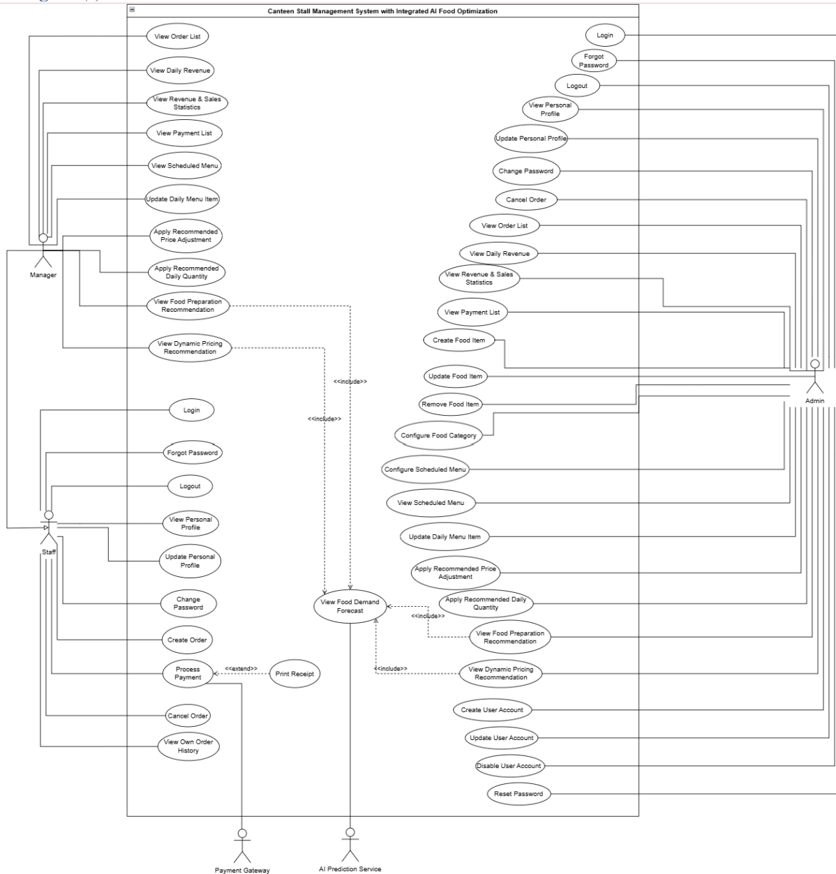
Figure 1. Use Case Diagram Overview
