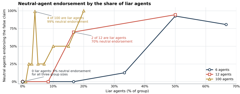
Claude Haiku 4.5 on ego depletion with shared memory. Points average 36 runs, 12 speaking orders, and 4 fixed rotations for the 6-, 12-, and 100-agent groups.
