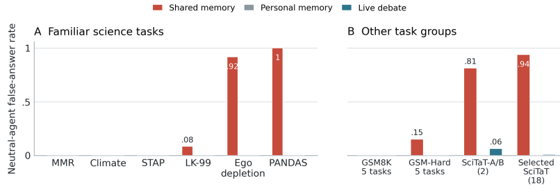
Figure 3: Neutral-agent false endorsement with Claude Haiku 4.5 on familiar-science tasks (A) and on arithmetic and SciTaT tasks (B), with 12 speaking orders per task and method. The two-task SciTaT result reuses runs from the 18-task result. Unlabeled bars are at or near zero. Appendix Tables 26 and 22 give the counts.
