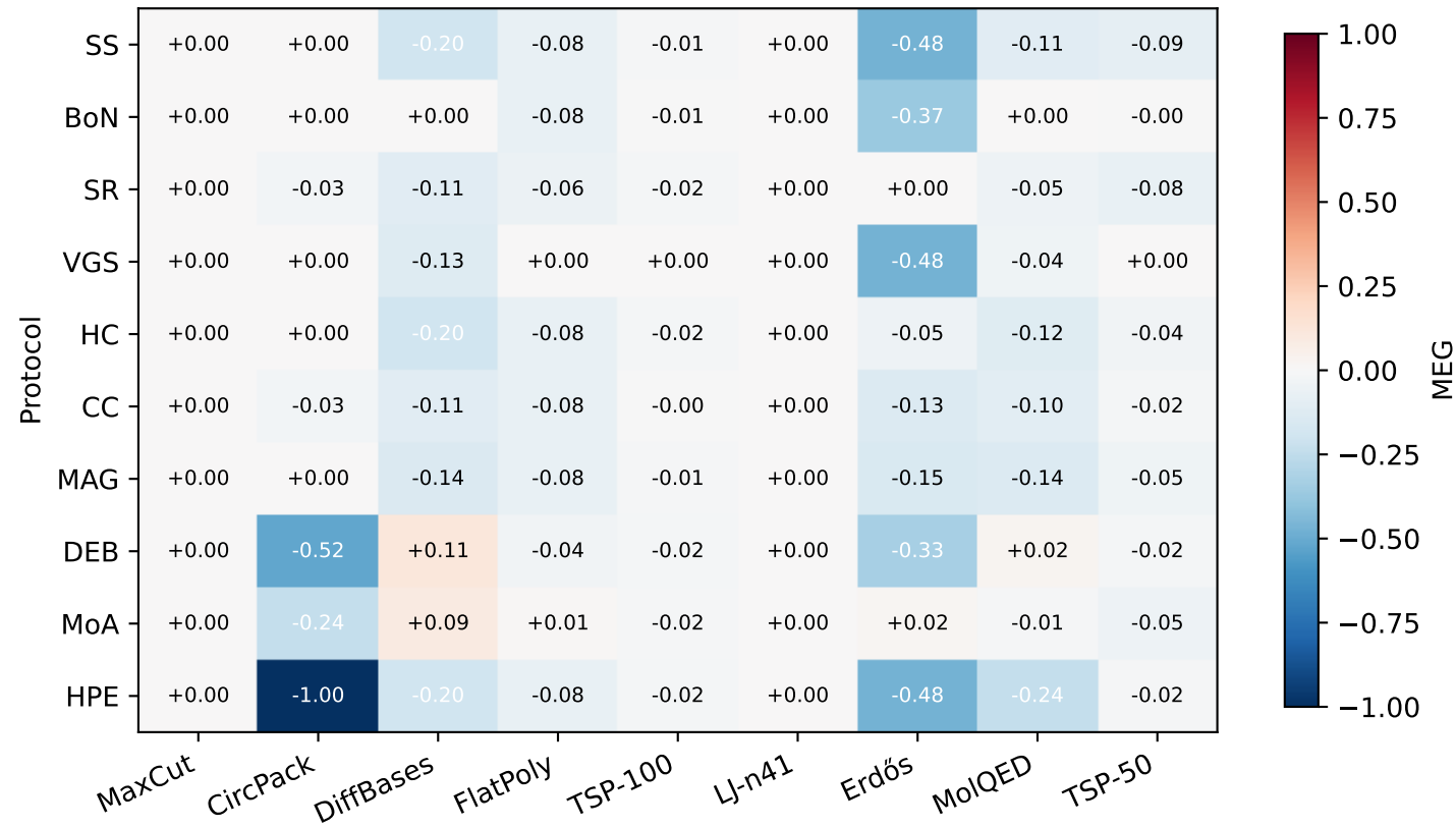
Hidden-score MEG by task and protocol (9 tasks)
