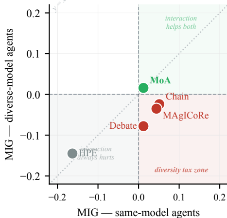
(b) Interaction erases diversity
