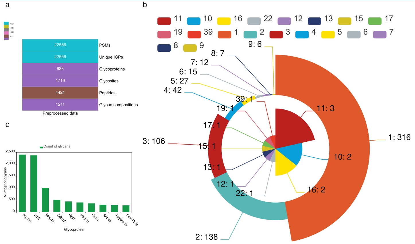
a: Overall profiling of preprocessed glycoproteomics data. b: Number of glycoproteins grouped by the count of glycosylation sites. c: Top 10 glycoproteins ranked by the number of glycan across all glycosylation sites.
