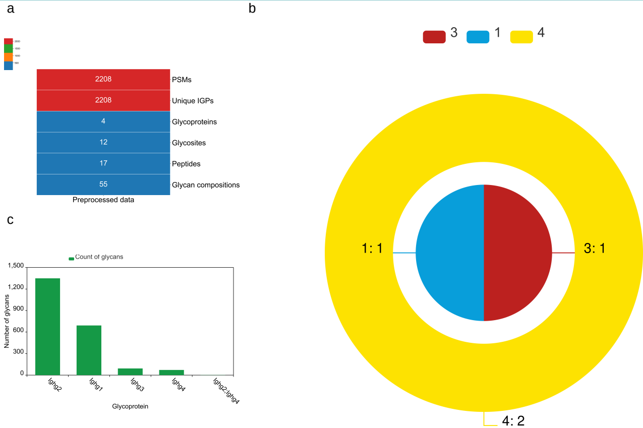
a: Overall profiling of preprocessed glycoproteomics data. b: Number of glycoproteins grouped by the count of glycosylation sites. c: Top 10 glycoproteins ranked by the number of glycan across all glycosylation sites.
