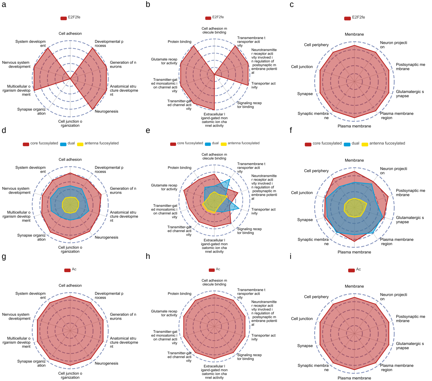
a: Distribution of different LacdiNAc across the top 10 GO:BP-enriched terms. b: Distribution of different LacdiNAc across the top 10 GO:MF-enriched terms. c: Distribution of different LacdiNAc across the top 10 GO:CC-enriched terms. d: Distribution of different fucosylated types across the top 10 GO:BP-enriched terms. e: Distribution of different fucosylated types across the top 10 GO:MF-enriched terms. f: Distribution of different fucosylated types across the top 10 GO:CC-enriched terms. g: Distribution of different sialylated types across the top 10 GO:BP-enriched terms. h: Distribution of different sialylated types across the top 10 GO:MF-enriched terms. i: Distribution of different sialylated types across the top 10 GO:CC-enriched terms.
