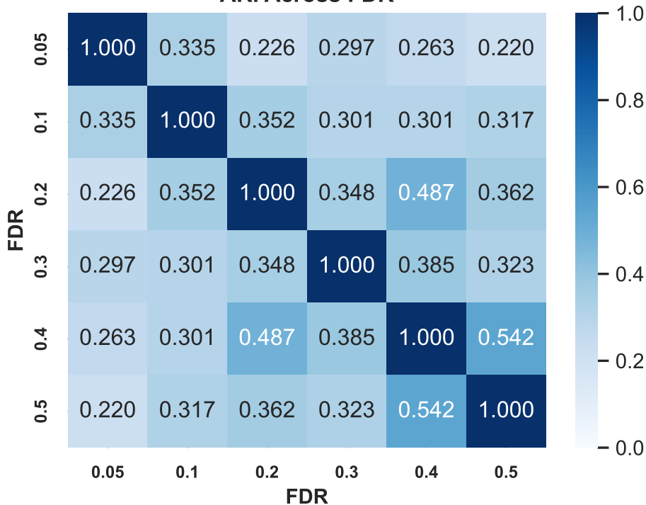
ARI Across FDR
