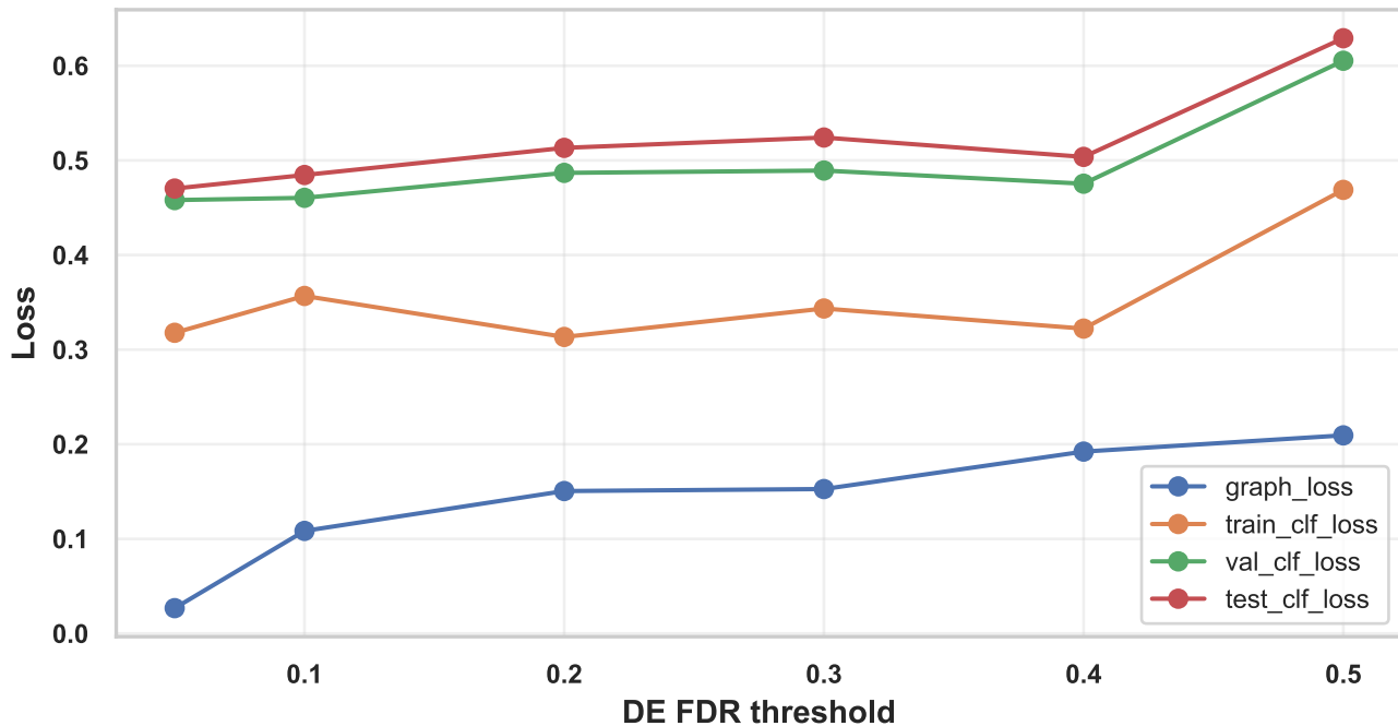
Post-hoc Loss Decomposition Across DE FDR Settings
