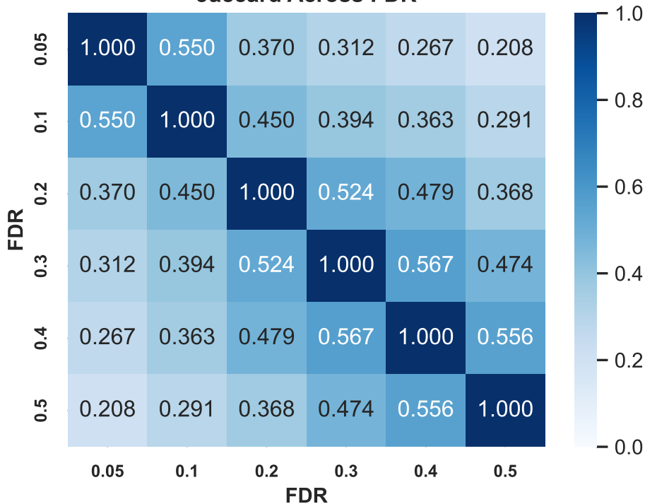
Jaccard Across FDR
