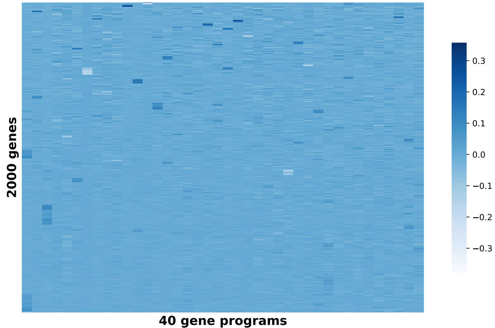
sciRED MicroPVM
