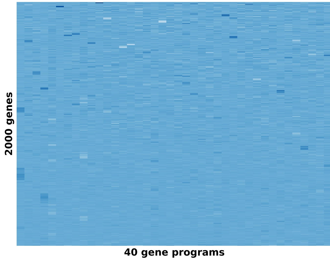
sciRED Astro
