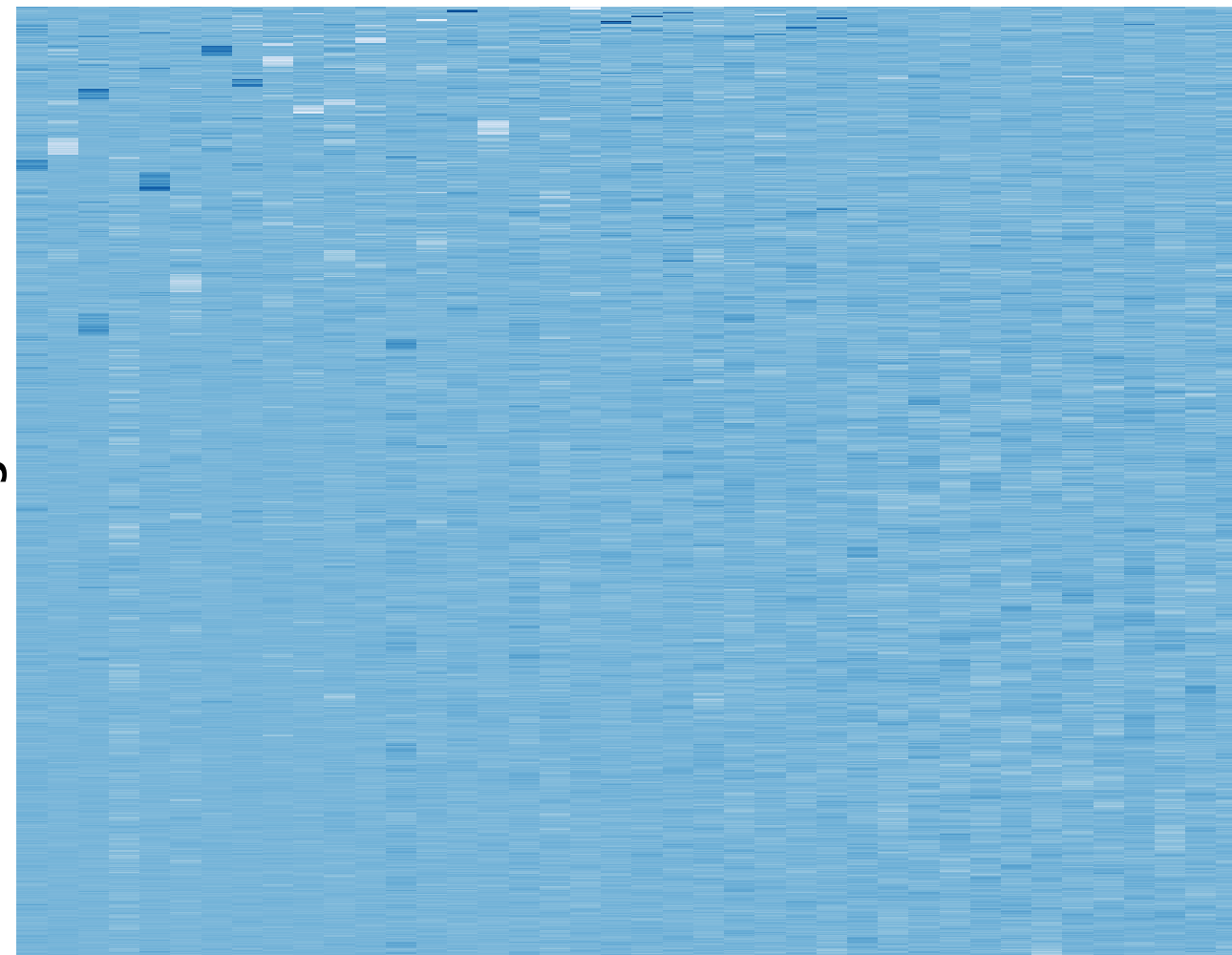
sciRED CD8
