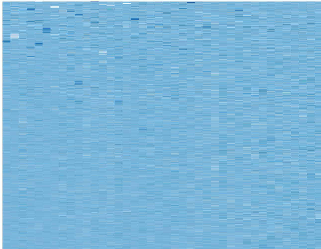
sciRED CD4
