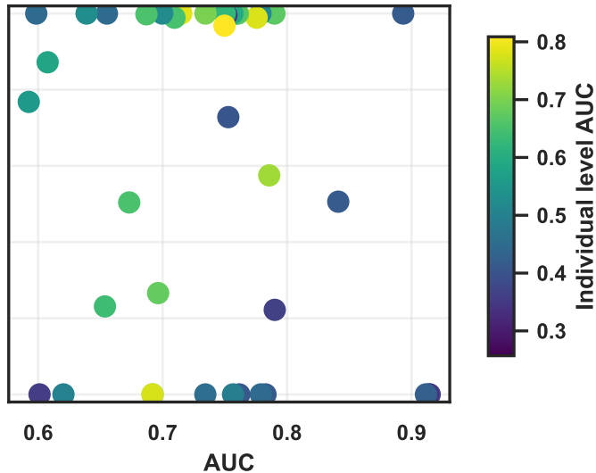
Spectra Micro-PVM
