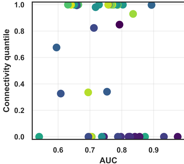
Spectra Astro
