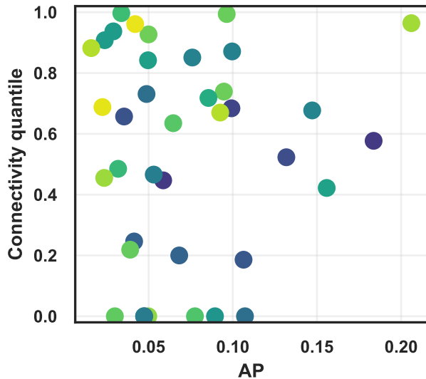
Spectra CD4
