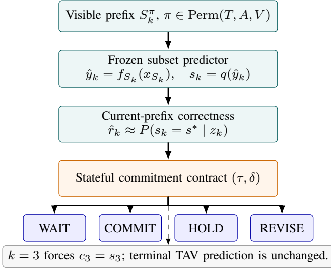
Fig. 1. The AMAC interface. Modalities arrive in an arbitrary order. A frozen predictor produces a state for each visible prefix, the prefix-correctness estimator scores its probability of being correct, and the contract chooses WAIT, COMMIT, HOLD, or REVISE. Clip index i is omitted in the diagram. The third modality forces the complete TAV state.
