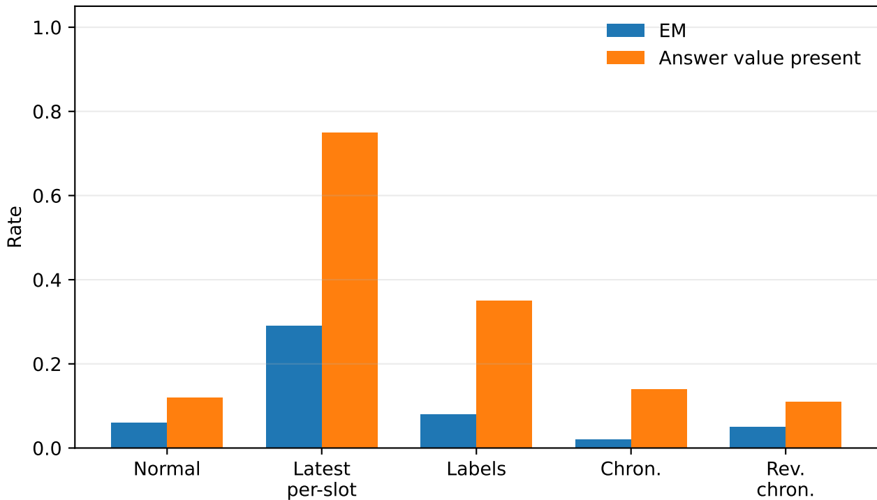
Llama3.1-8B stale susceptibility
