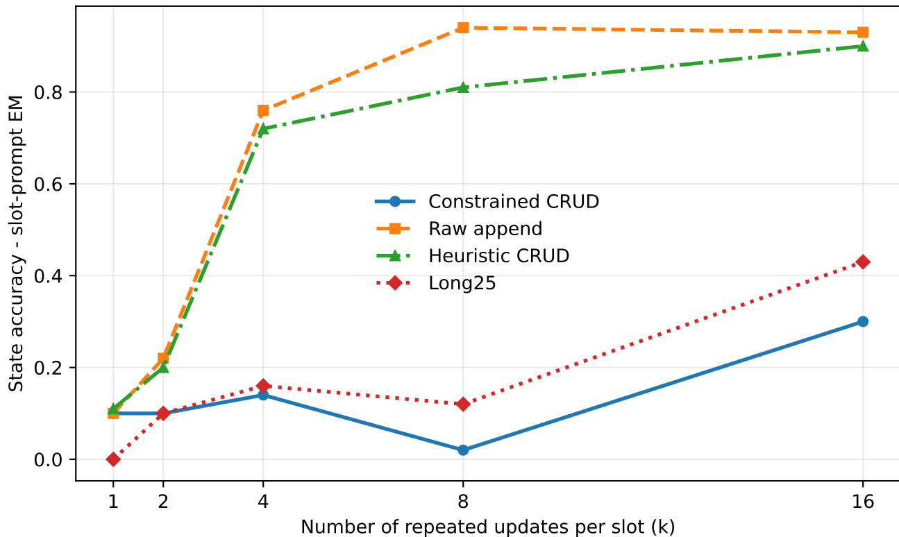
Oracle-state vs slot-prompt gap
