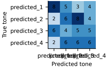
wav2vec2
