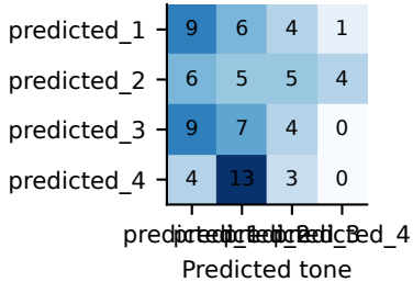
Acoustic
