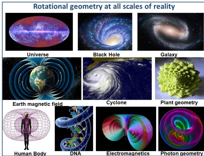
Figure 2: Geometry of the “Torus”, present on various scales in the Universe
