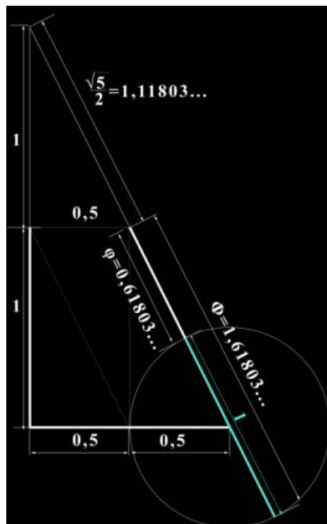
Figure 1. Pythagoras' secret on the left, and on the right the numbers of the sequences connected to that of Fibonacci
