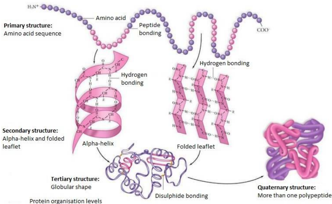
Figure 4 - Image downloaded from thechimica-online.it website, the secondary and tertiary structure of proteins.
