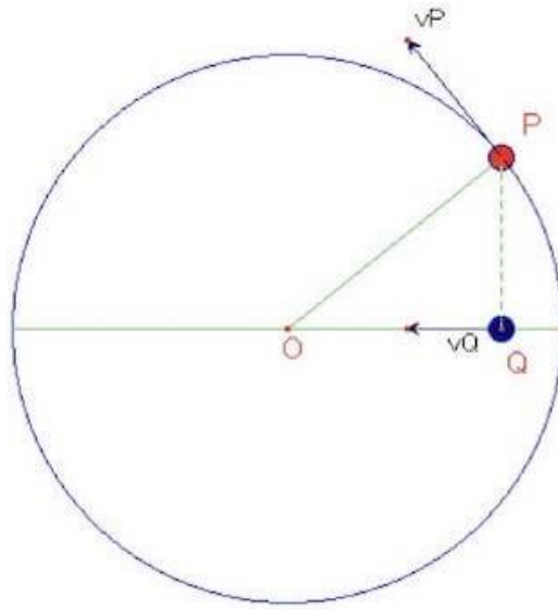
Figure 5. Harmonic movement ( https://www.chimica-online.it )
