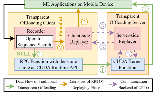
Fig. 4: Architecture of RRTO, with key components highlighted in red boxes.
