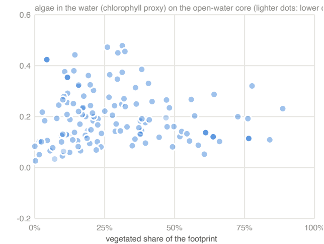
Assessed lakes with a computable chlorophyll proxy: vegetated share against the chlorophyll proxy on the open-water core, reading window medians. Two groups: mat-covered lakes and bloom-prone open lakes; both are eutrophication, with different measures.
