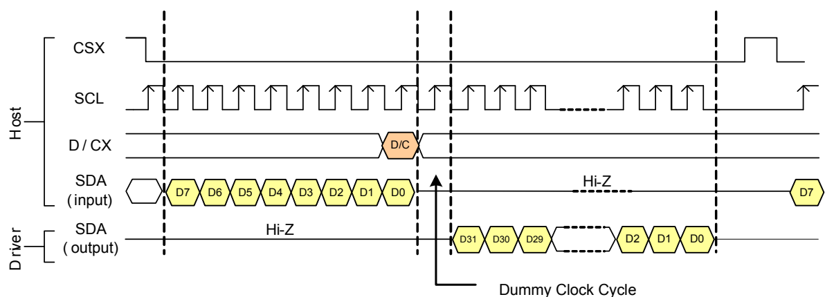
Figure 10: DBI Type C (Option 3) Read Cycle Sequence
