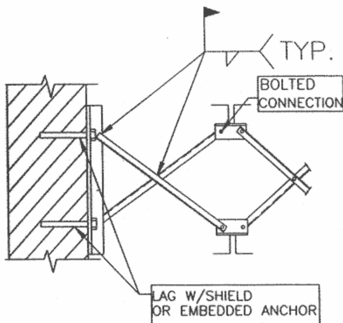
BOLTED DIAGONAL BRIDGING TERMINUS AT WALL
