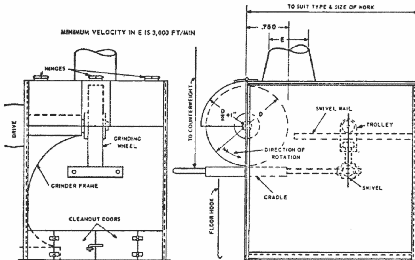
FIGURE D-57.5—CRADLE POLISHING OR GRINDING ENCLOSURE
