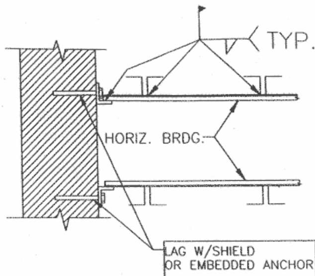
HORIZONTAL BRIDGING TERMINUS AT WALL
