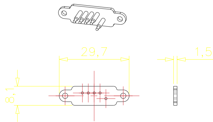
Cybertel PCB
