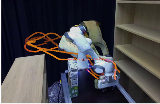
Fig. 10. Example of multimodal trajectories executed in the warehouse environment using MPD. Starting from the same joint configuration, the task is to reach an end-effector pose on the table while avoiding collisions with the environment. The orange lines depict the end-effector trajectories, and the overlaid images show the last frame on the trajectory. Our model generates multiple goal robot configurations for similar desired end-effector poses.
