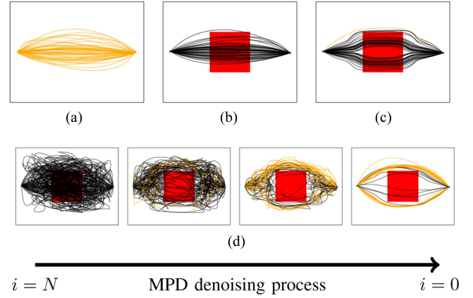
Fig. 11. Benefits of sampling with MPD instead of first sampling from the prior and then optimizing the cost function. (a) The robot is a 2-D point mass in an environment without any obstacles, and demonstration trajectories are obtained by sampling from a GP prior. At inference, an obstacle (in red) is inserted into the environment. (b) Samples from the learned diffusion prior. (c) Results of first sampling from the prior and then optimizing the collision cost function. (d) Samples from the posterior distribution generated with MPD. The second row illustrates how MPD's denoising process moves from Gaussian noise to clean trajectories while avoiding the red obstacle. Trajectories that are in collision with the red obstacles are shown in black, and collision-free trajectories in orange. (a) Demonstrations. (b) Dprior. (c) Dprior + Cost. (d) MPD.
