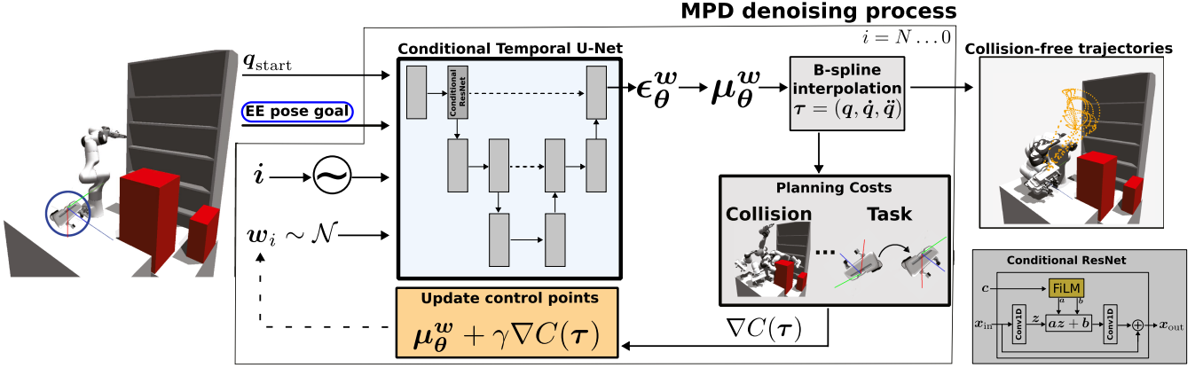
Fig. 2. Overview of inference using MDP. An initial joint position q_{\text{start}} and an end-effector goal pose {}^W H_{\text{goal}}^{EE} \in SE(3) are context variables to a conditional diffusion model. The diffusion model consists of a conditional U-Net architecture (made of conditional ResNet blocks) that takes as input the context, the current time index i and the B-spline control points w_i , and outputs the denoising vector \epsilon_\theta . The control points mean \mu_i are obtained with (6) and used to compute the gradient of a motion planning cost function, which is used to bias the samples toward higher (negative) cost likelihood regions. These particles are injected as input to the U-Net at the next denoising step. In the conditional ResNet block, the time and context embeddings are stacked and used as input for computing the parameters a and b of a FiLM encoder, which are used to transform the embedded control points ( x_{\text{in}} ), computed with a 1-D convolution. MPD's output are joint space trajectories that balance the prior distribution and the cost likelihood.
