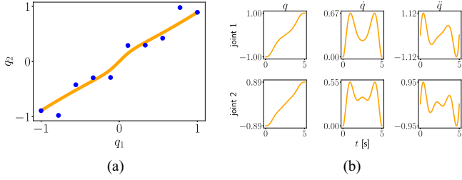
Fig. 3. Resulting trajectories when using linear phase-time scaling. In (a), the control points (blue dots) and path of a clamped fifth-order B-spline are displayed. (b) shows the trajectory in time of positions, velocities, and accelerations for the two degrees of freedom. (a) Control points and curve (b) Trajectories in time.
