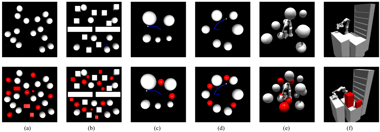
Fig. 5. Environments used for the motion planning experiments, with different robot models and increasing complexity. In 2-D tasks the robots are depicted in blue (as a dot for RobotPointMass2D). The bottom row shows the tasks with additional obstacles (in red), which are not present during training. (a) EnvSimple2D-RobotPointMass2D. (b) EnvNarrowPassageDense2DRobotPointMass2D. (c) EnvPlanar2Link-RobotPlanar2Link. (d) EnvPlanar4Link-RobotPlanar4Link. (e) EnvSpheres3D-RobotPanda. (f) EnvWarehouse-RobotPanda.
