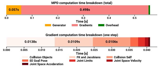
Fig. 7. Computation times breakdown for sampling 100 trajectories with MPD in the EnvSpheres3D-RobotPanda environment. (Top) MPD total inference time and breakdown per generator and gradient computations. (Bottom) Breakdown for the computation of one gradient step.
