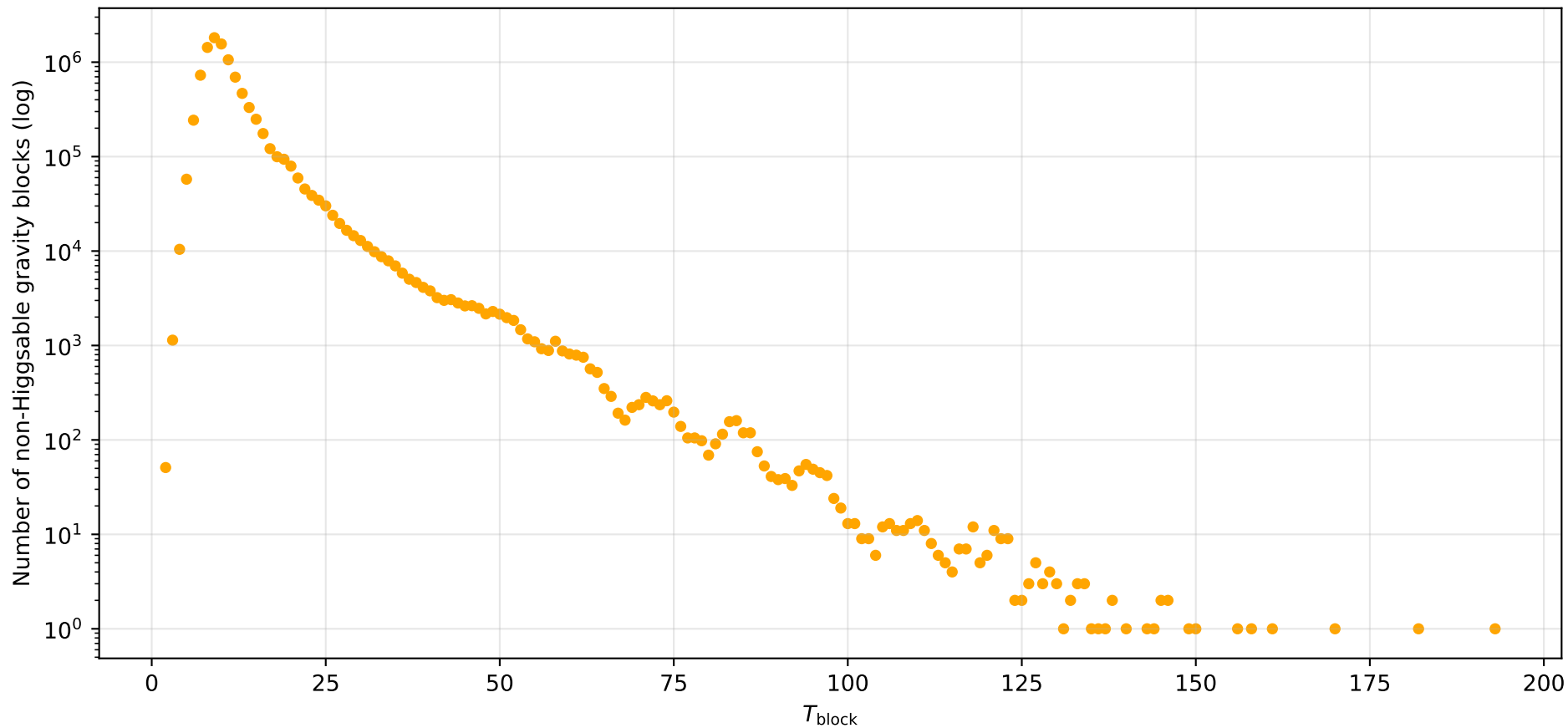
Non-Higgsable gravity blocks per T_{\text{block}}
