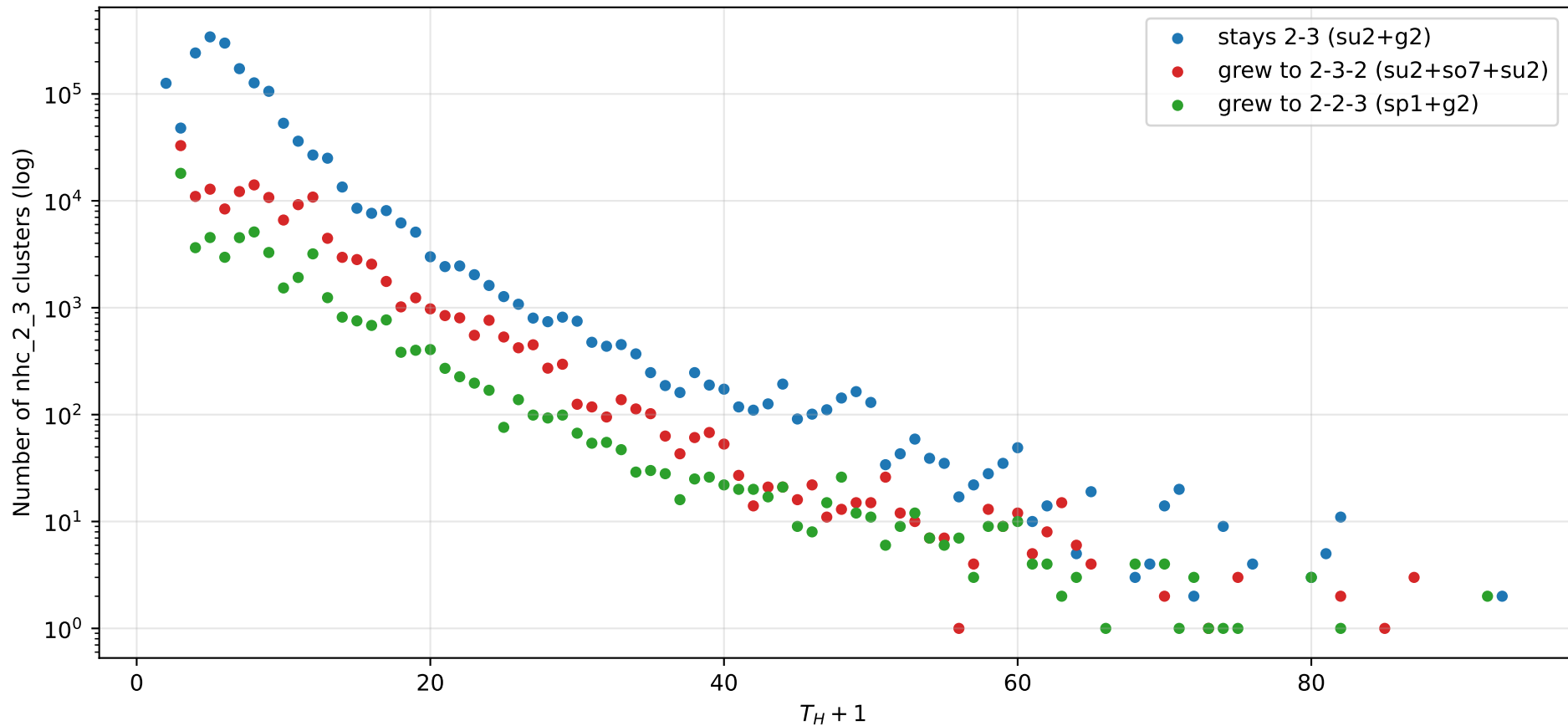
Fate of attached -2-3 clusters per T_H + 1
